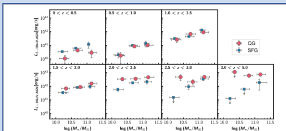
Figure: X-ray AGN luminosity as a function of redshift and stellar mass.
